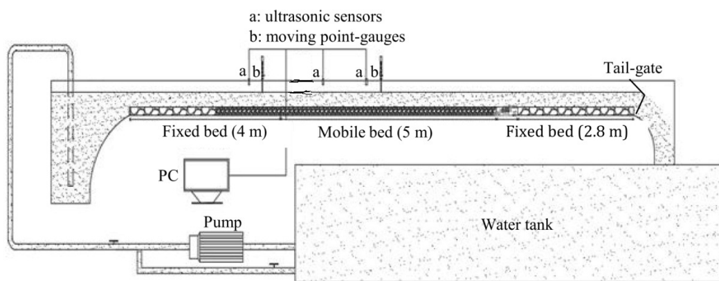
Figure 1. Experimental flume set-up (not to scale) [29].
