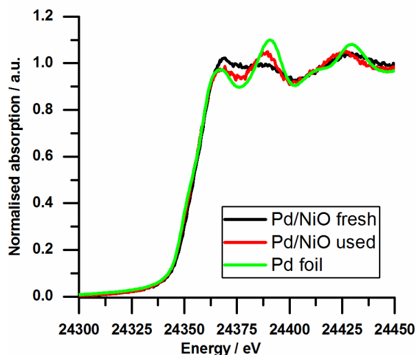
13 14 15 16 17 18 19 20 21 22 23 24 25 26 27 28 29 30 31 32 Figure 7. Pd K edge XANES of 1% Pd/NiO before and after reaction and a reference Pd foil.
