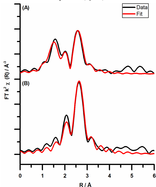
30 31 32 33 34 35 36 37 38 39 40 41 42 43 44 45 46 47 48 49 50 51 52 53 54 55 56 57 58 59 60 Figure 8. k 2 weighted Fourier transform EXAFS data with simulated fit for (a) the fresh Pd/NiO and (b) the used Pd/NiO.
