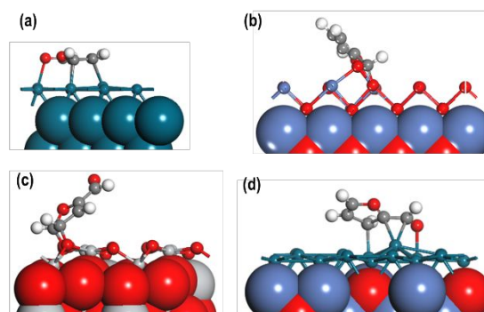
Figure 4. The optimized structures of furfural adsorbed on (a) Pd(111), (b) NiO(110), (c) TiO 2 (111) and (d) Pd 16 /NiO(110) surfaces. For clarity, the furfural molecule and the first two layers of the surfaces are shown as ball and stick and lower layers are shown in the CPK format.
