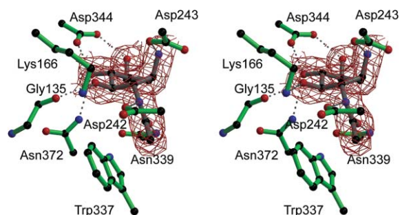
Fig. 2 Observed electron density for 7 binding to Bt GH84 shown in divergent (wall-eyed) stereo; 7 is shown in grey and with observed 2F_{\text{obs}} - F_{\text{calc}} electron density at 0.4 electrons \text{\AA}^{-3} . Interacting amino-acids discussed in the text are shown and are coloured green.
