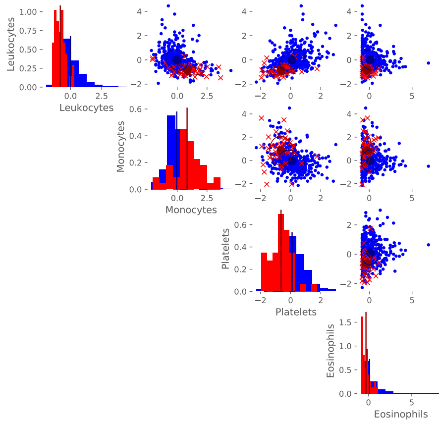
Suppl. fig. 1: Scatter plots corresponding to the top four features of patients not admitted to hospital (community); categorized by whether tested positive (red) or negative (blue) to rt-PCR SARS-CoV-2 test. Dark colours represent averages and error covariance ellipses correspond to 1 standard deviation.
