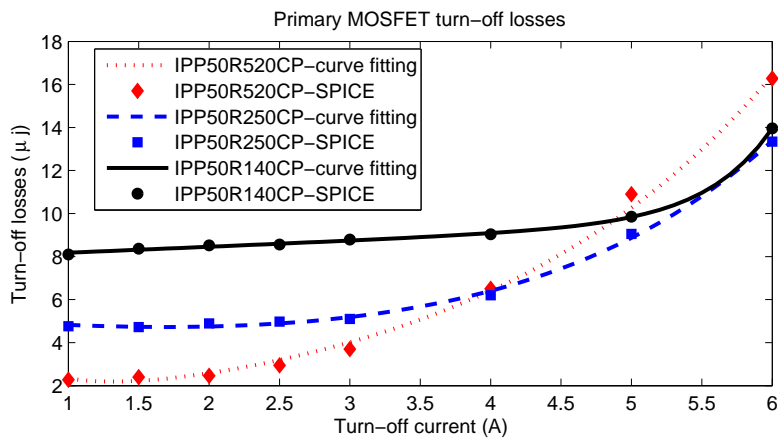
Fig. 5. PSPICE simulated primary MOSFET turn-off loss.
