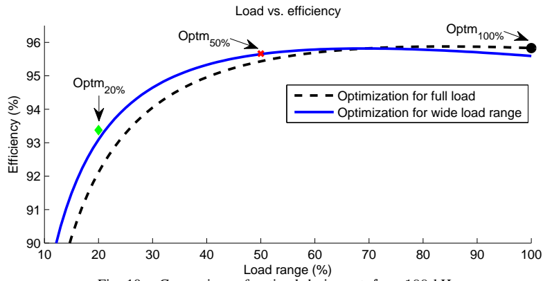
Fig. 10. Comparison of optimal designs at f_s = 100 kHz.
