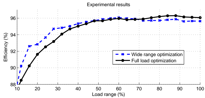
Fig. 13. Experimental efficiency comparisons, V_{in} = 370V .
