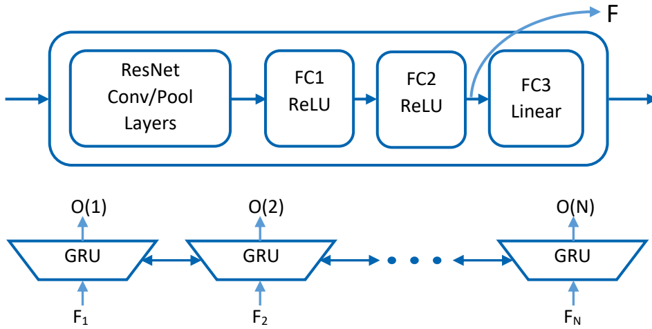
Figure 5. The CNN part of the CNN-RNN architecture feeds the RNN part which yields the final outputs
