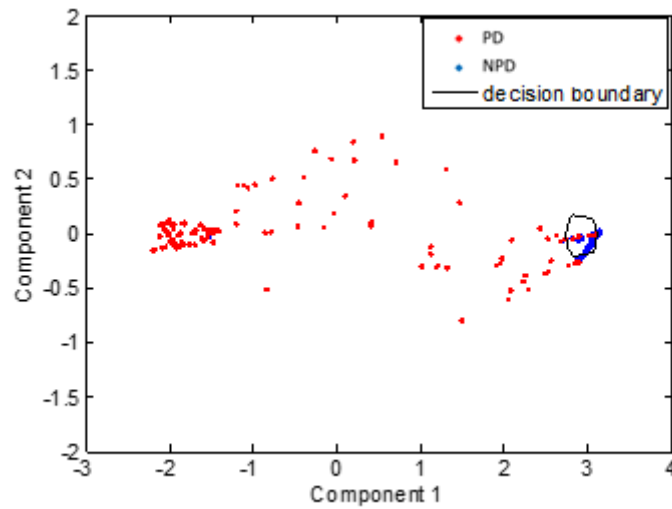
Figure 12b. Visualization of (one) cluster boundary for the NPD category provided by an OCSVM approach.
