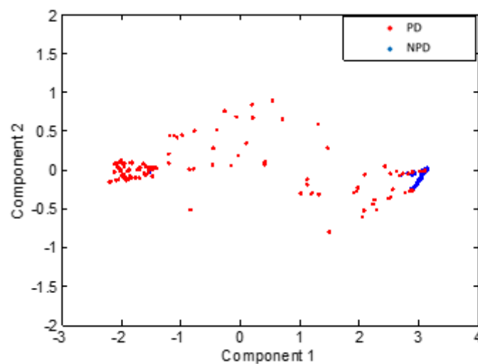
Figure 12a. The two main principal components of the CNN-RNN representation.
