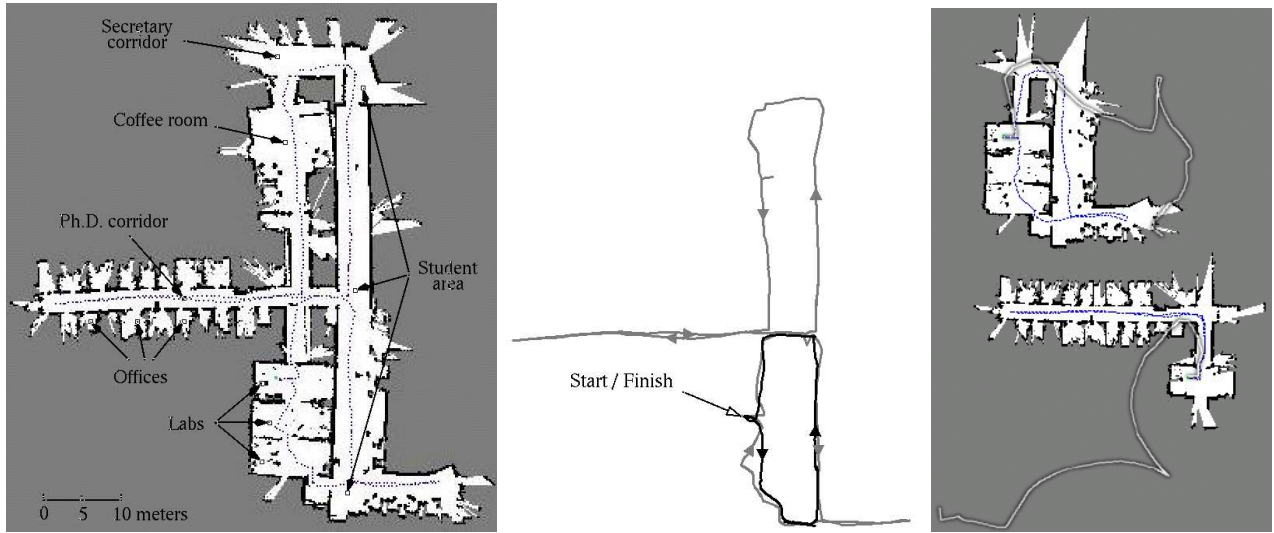
Fig. 6. Left: area covered by the database. Middle: ground truth information from SLAM, Run 4 (black) and the database (gray). Right: Two of the test sequences with ground truth and raw odometry data, Run 1 (above) and Run 2 (below).
