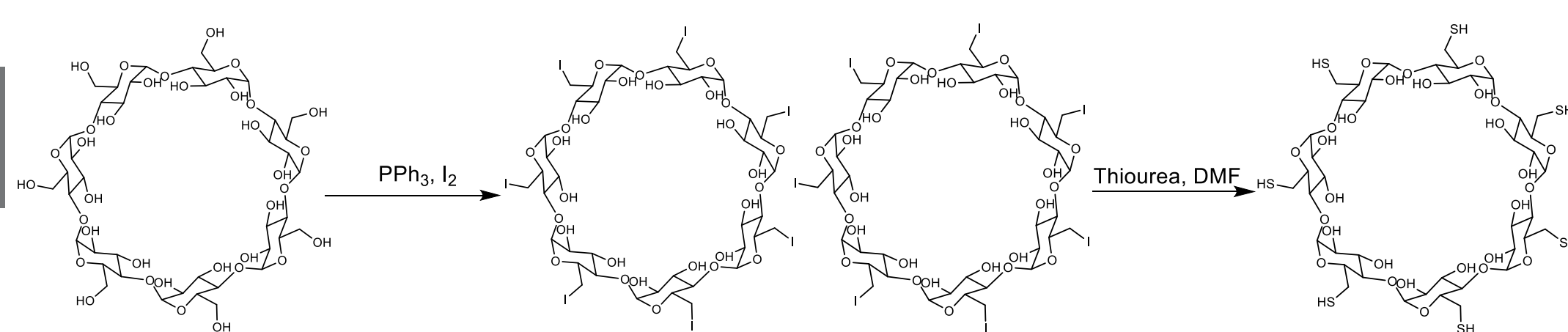
Figure 4. Synthesis of iodinated CD with triphenylphosphine and iodine, followed by the thiolation with thiourea and DMF.
