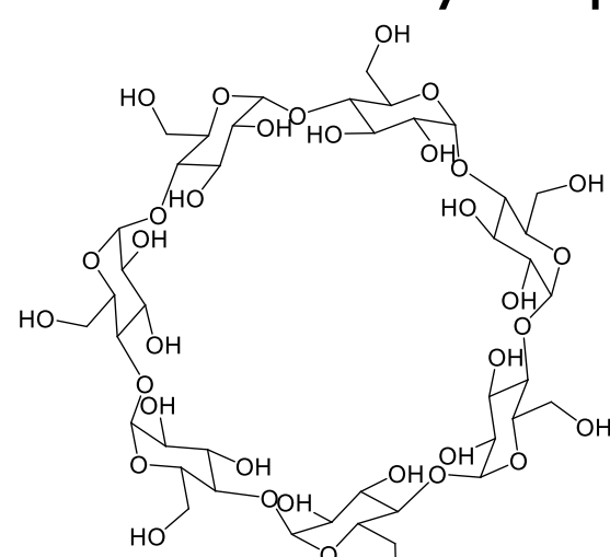
Figure 1. CD macrocycle structure.
