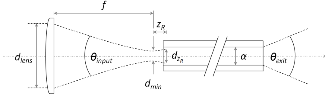
Figure 2: Schematic of HCW launch/exit configuration. The dashed lines represent the marginal rays whereas the dashed-dot line represents the optical axis.
