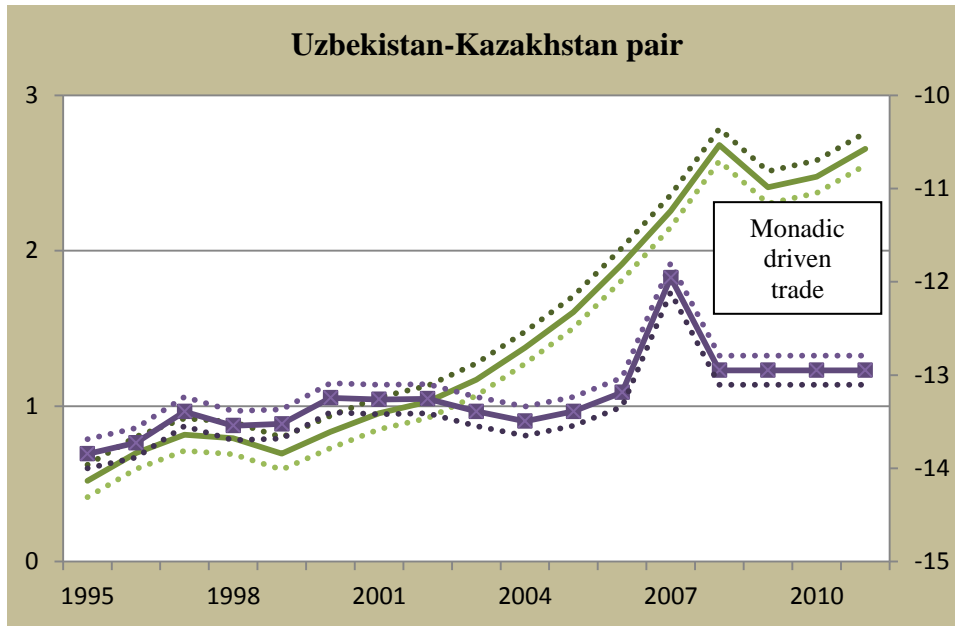
Figure 2 Illustrative examples of Monadic-driven and Dyadic-driven trade
