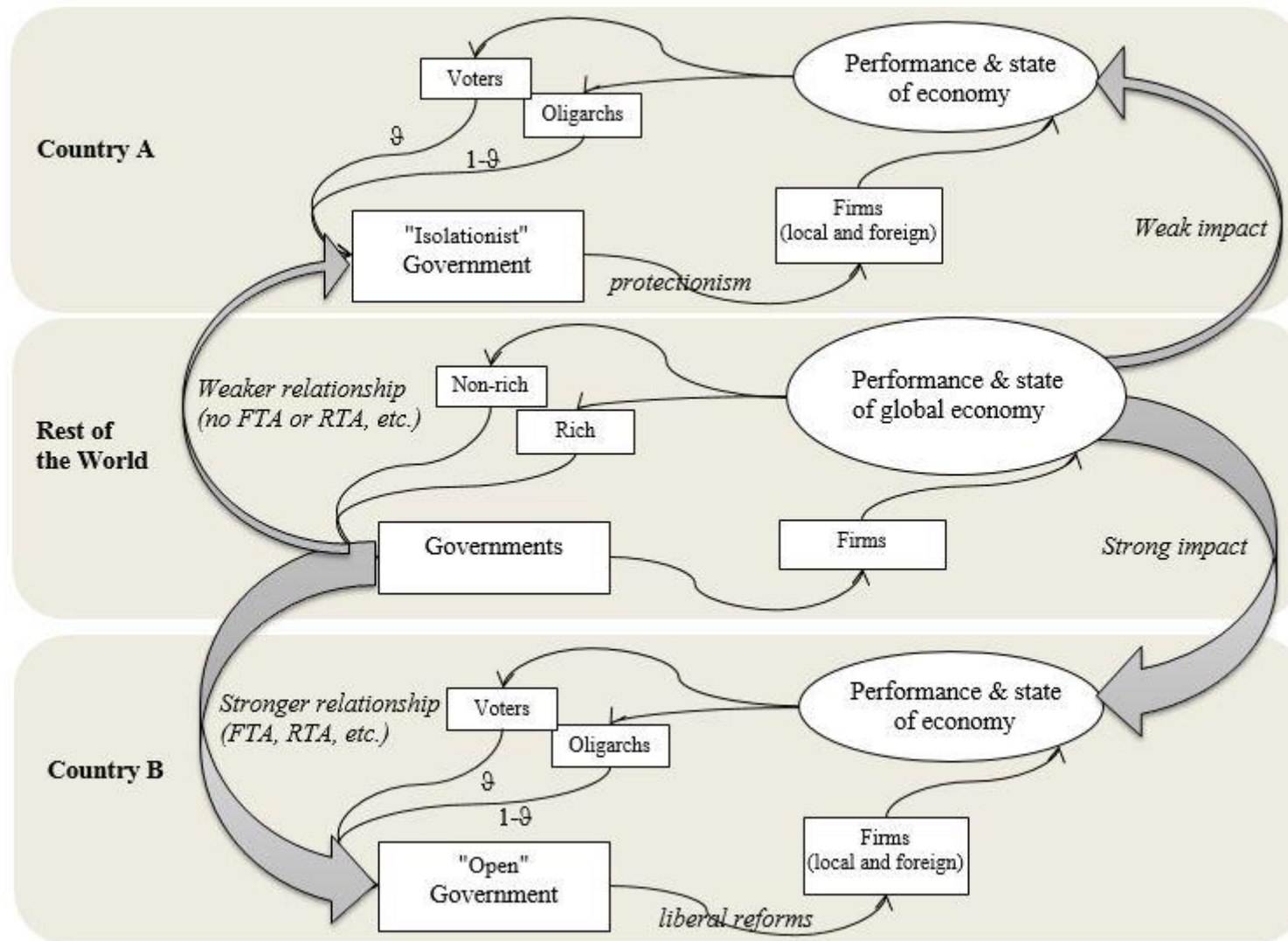
Figure 1 A game tree of openness and trade: actors and interactions
