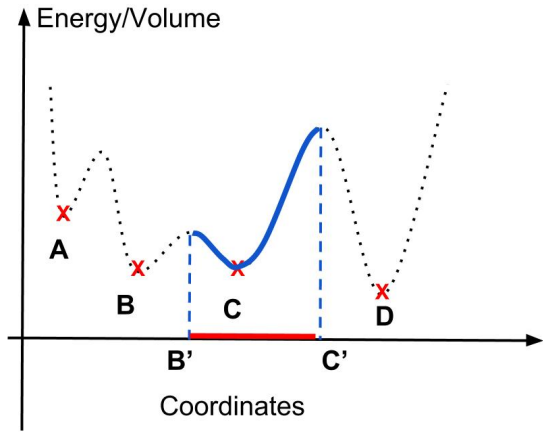
Figure 1. (Color online) Schematic representation (dotted line) of an energy or volume landscape that can be used to generate four mechanically stable packings (A, B, C, D). For each minimum, it is not possible to decrease further the cost function without first increasing the volume available (volume landscape interpretation like the LS algorithm) or the energy of the system (energy landscape interpretation). The solid blue line represents the basin of attraction of the minimum C while the length of the red segment B'C' represents its size. In a multidimensional space, this size becomes a hyper-volume in the space of coordinates.
