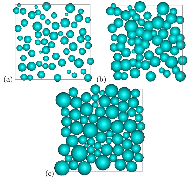
Figure 2. Jammed state as generated by potential energy minimization. One starts by picking a state (a) from an equilibrated hard-sphere fluid. Then, the soft shell interaction is turned-on and the packing fraction is now such that there are many overlaps (b). The system relaxes then to the corresponding potential energy minimum, yielding the jammed state (c).
