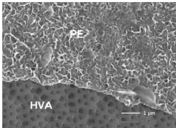
Fig. 6. SEM of Coscinodiscus perforatus cell to show hypoalveolate areolation (HVA) and overlying perfrustular envelope (PE). Reworked detail from Beninger and Decottignies (2009).
