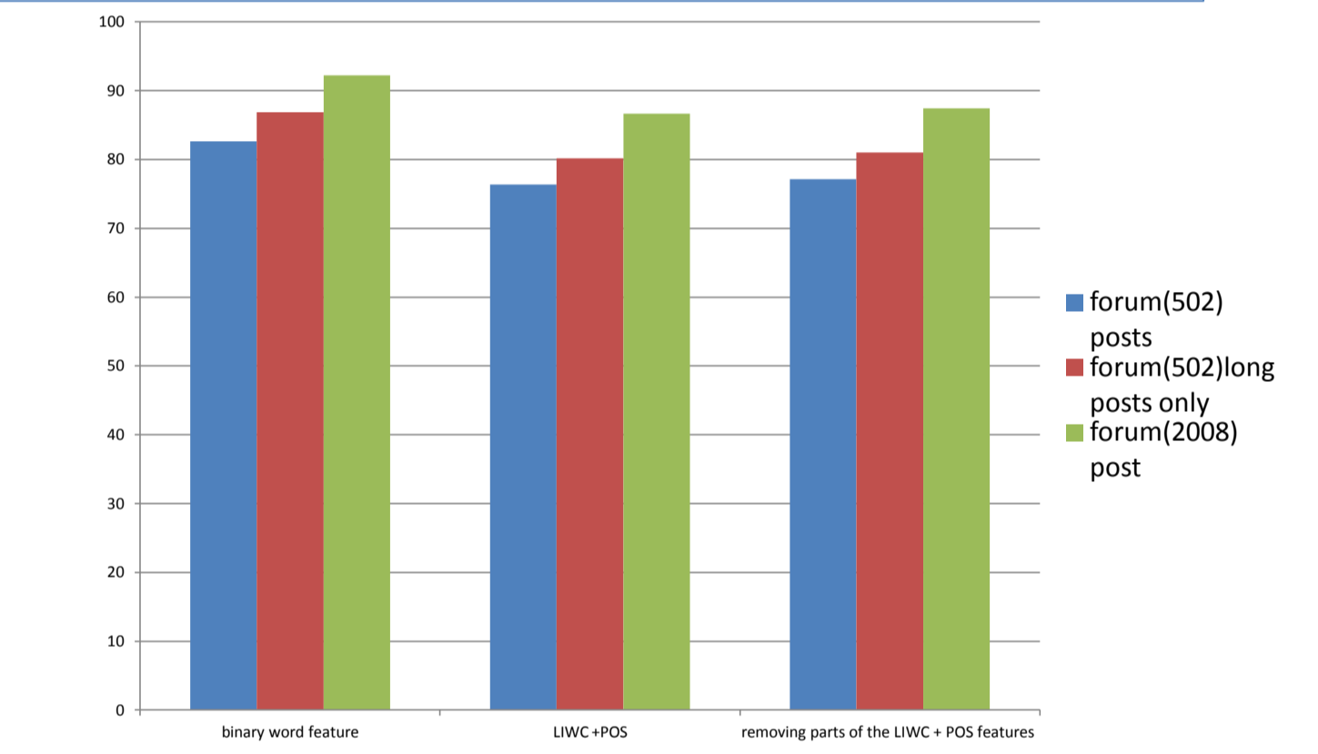
Figure 2. Forum Data Classification Accuracy With Different Features
