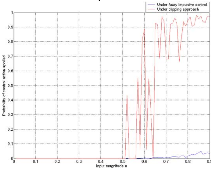
Figure 8: Probability of control force applied to the SDM when the input sinusoidal frequency is \frac{2}{3} of the passband bandwidth, initial condition \tilde{\mathbf{x}}(0)=[0, 0, 0, 0, 0]^T and the state variables are bounded by 28.
