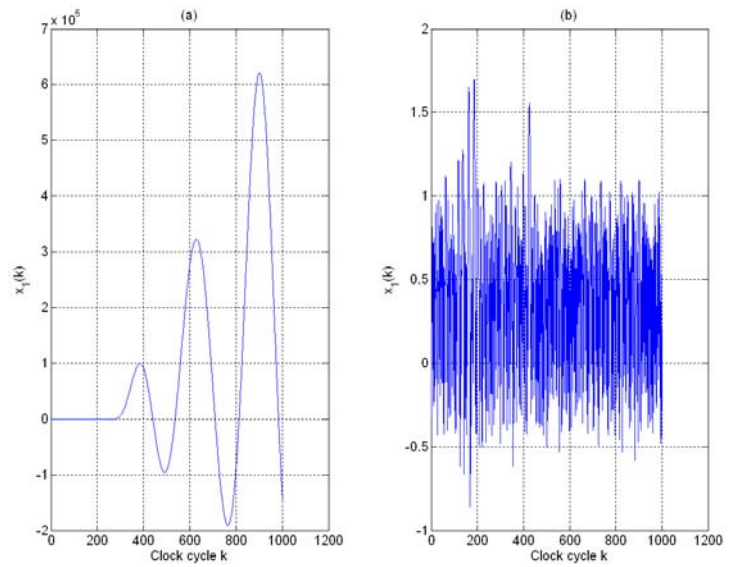
Figure 9: The response of x_1(k) with initial condition \tilde{\mathbf{x}}(0)=[0, 0, 0, 0, 0]^T and input step size \bar{u}=0.59 (a) when no control strategy is applied. (b) when the fuzzy impulsive control strategy with V_{cc}=2 is applied.
